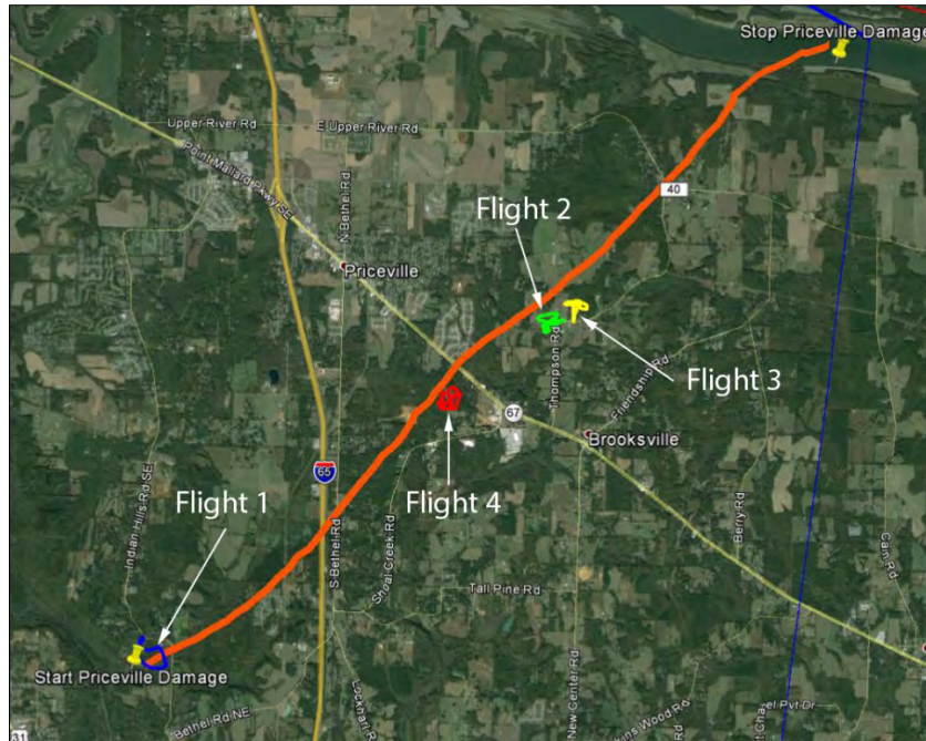
Figure 9: EF-2 tornado damage path (thick orange line) near Priceville on 31 March 2016 and sUAS flights on 5 April 2016. Flights 1, 2, 3, and 4 correspond with blue, green, yellow, and red lines, respectively.
